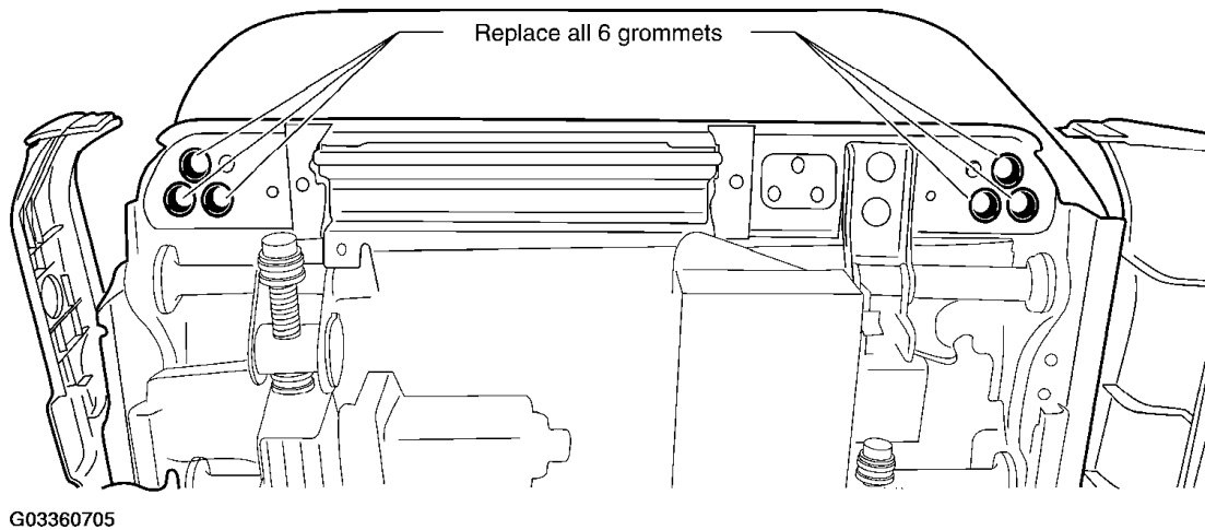
Fig. 10: Replacing All Six Rubber Grommets From Kit
