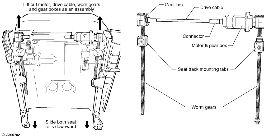
Fig. 7: Removing Worm Gears, Drive Cable, Motor & Gear Boxes
