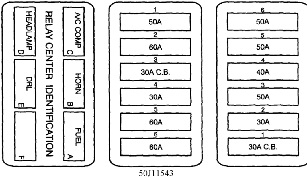
Fig. 2: High-Current Fuse Panel ID (1994-95 Seville) Courtesy of GENERAL MOTORS CORP.
