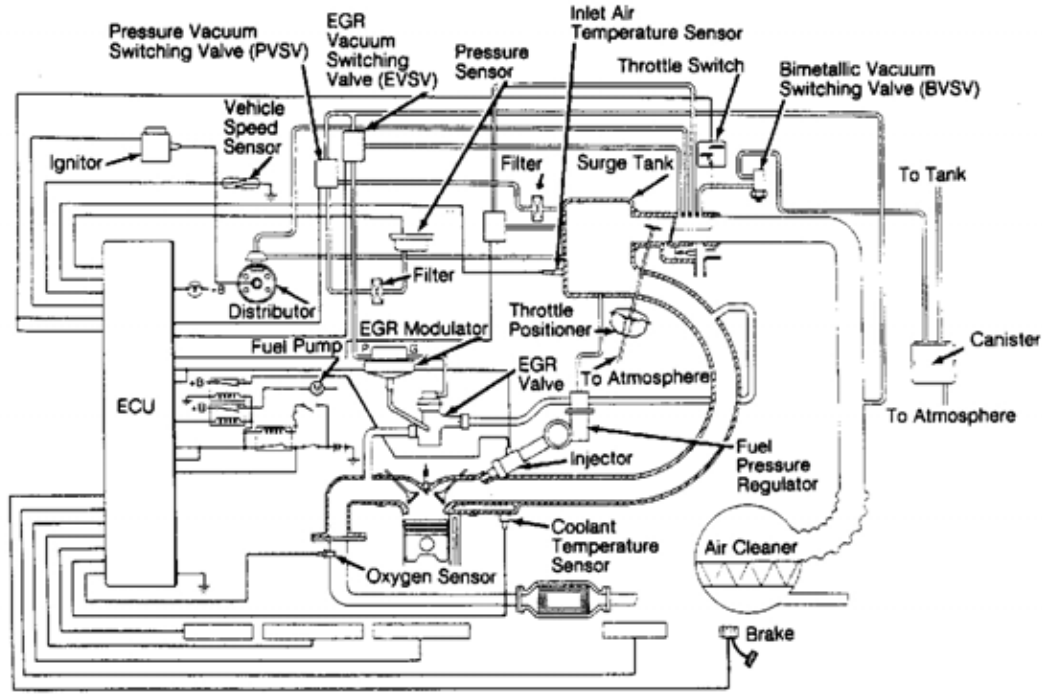
Fig. 4: Rocky 1.6L Vacuum & Component Diagram Courtesy of DAIHATSU MOTOR CO. LTD.
