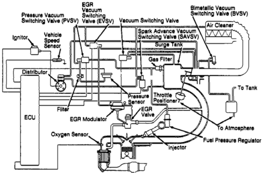
Fig. 3: Charade 1.3L Vacuum & Component Diagram (Manual Transmission) Courtesy of DAIHATSU MOTOR CO. LTD.
