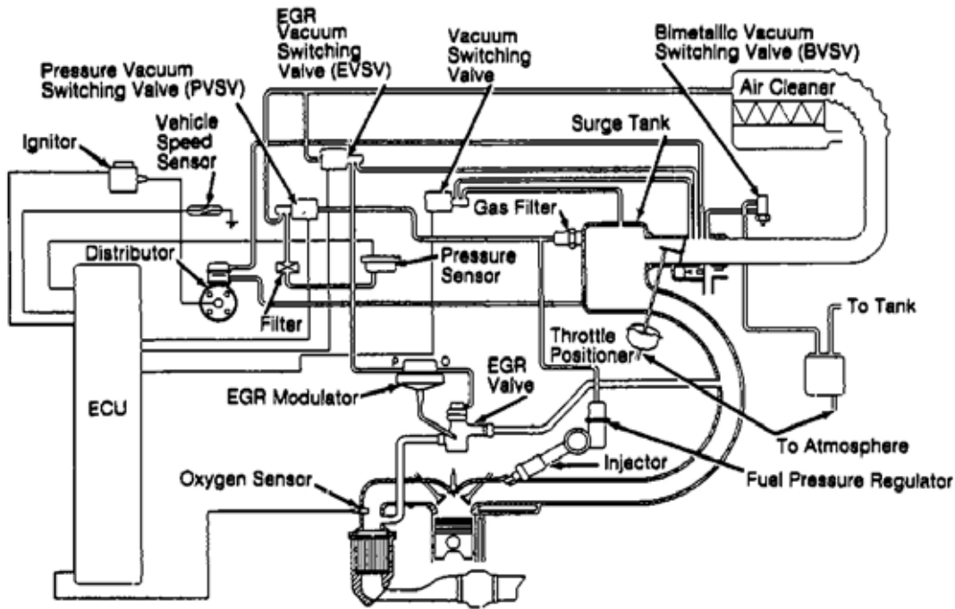
Fig. 2: Charade 1.3L Vacuum & Component Diagram (Automatic Transmission) Courtesy of DAIHATSU MOTOR CO. LTD.
