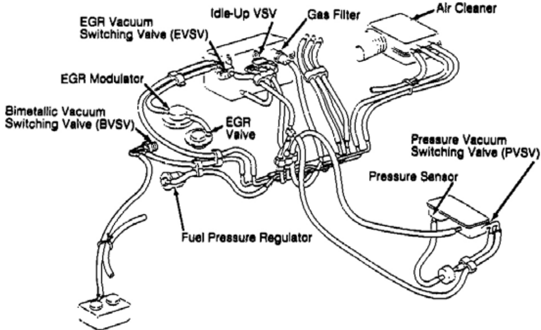
Fig. 1: Charade 1.0L Vacuum & Component Diagram Courtesy of DAIHATSU MOTOR CO. LTD.
